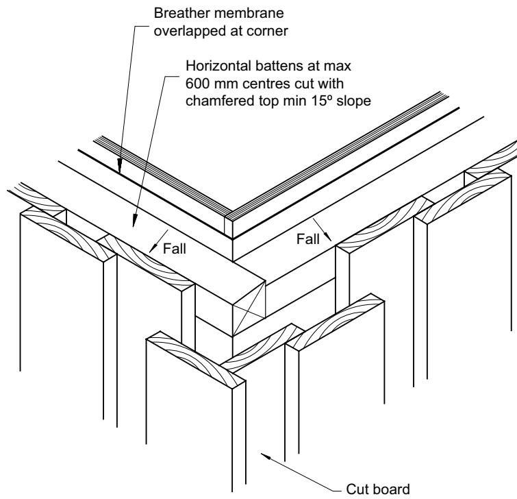
Figure 5.43 Typical corner detail in vertical board-on-board cladding
