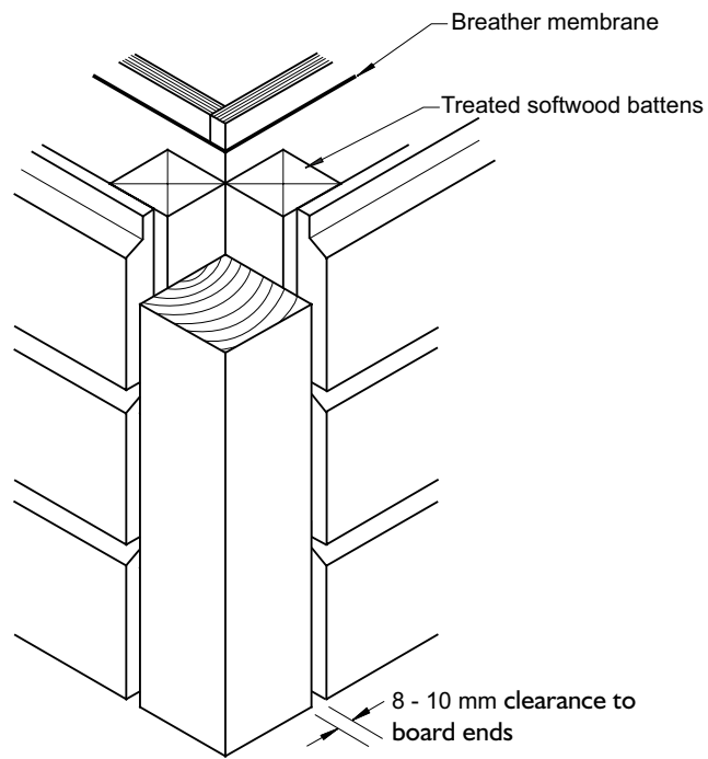
Figure 5.35 Solid timber corner detail in horizontal boarding
