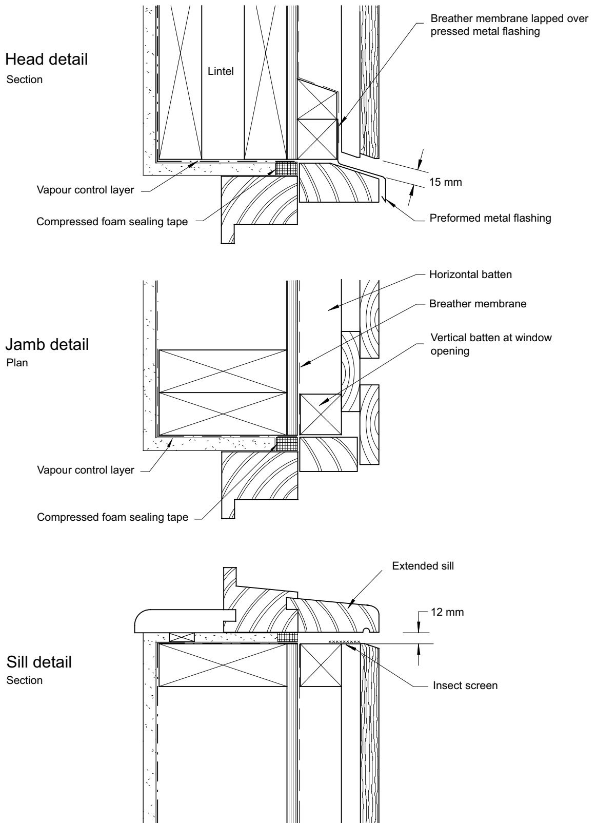
Figure 5.33 Typical detail of window in timber with vertical board-on-board cladding Note: A timber frame wall is shown: the detailing of the cladding with other forms of wall construction will be similar
