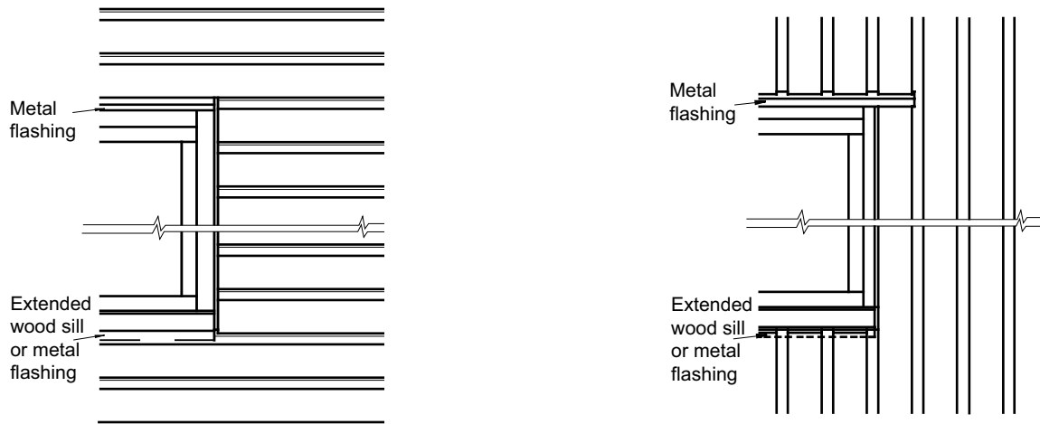
Figure 5.30 Typical elevation details of windows in horizontal boarding and vertical board-on-board cladding
