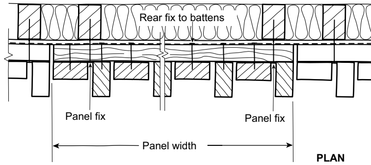
Figure 5.19 Vertical open jointed board on board
