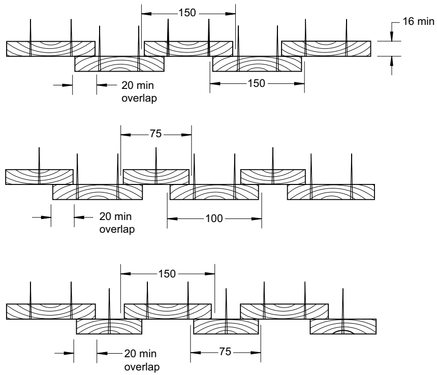
Figure 5.18 Profiles suitable for vertical boarding
