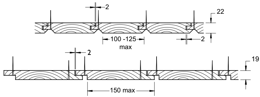
Figure 5.17 Profiles suitable for diagonal and vertical boarding
