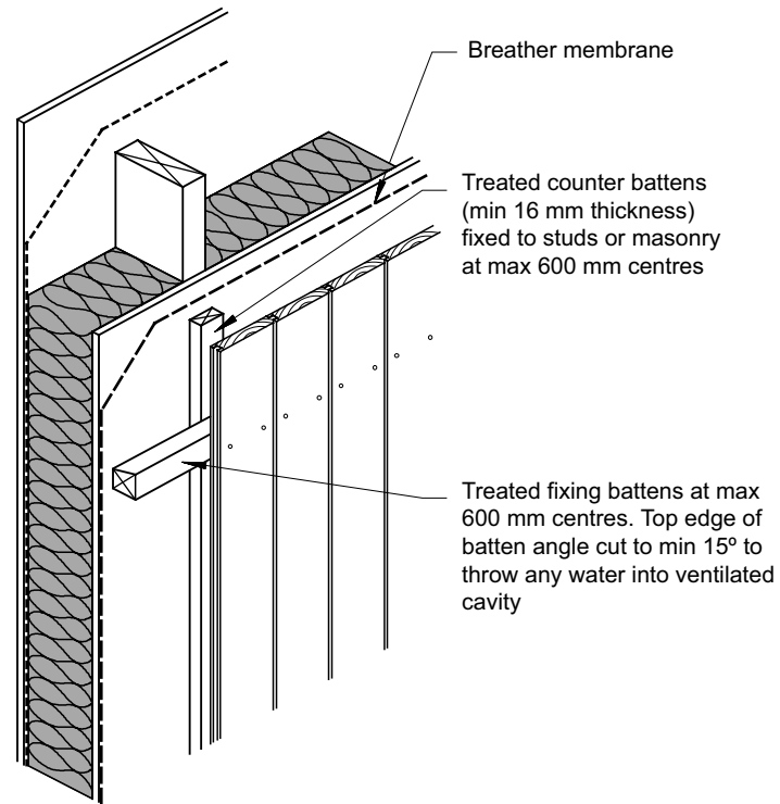
Figure 5.8 Typical construction: vertical tongued and grooved boarding on horizontal battens and counter battens
