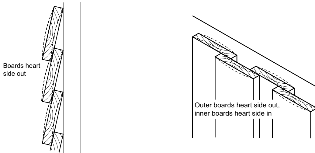
Figure 5.4 Exploiting the natural properties of timber Left: Horizontal boarding, Right: Vertical board-on-board cladding
